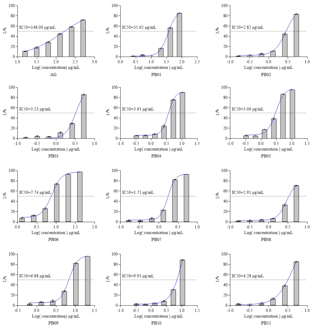
Figure S1 The IC 50 curves of AG and PB samples.
